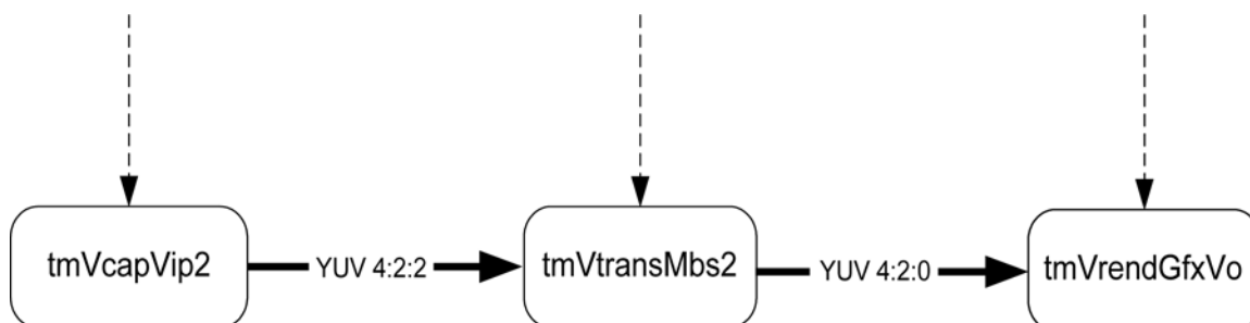
Figure 1: TSSA component graph for exoIVcodec
